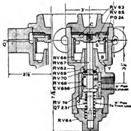
Fig. 2591. Accelerator Valve.
